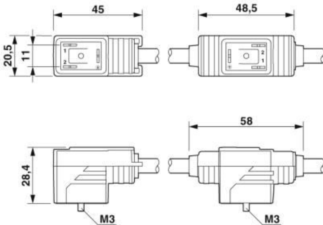
Double valve plug, 2 x type BI
