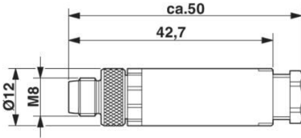
M8 x 1 male plug, straight version
