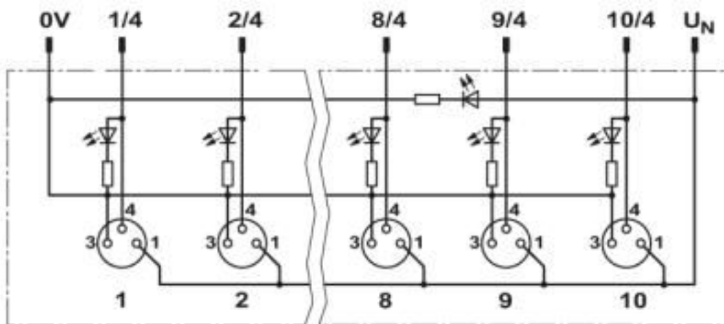
Circuit diagram
