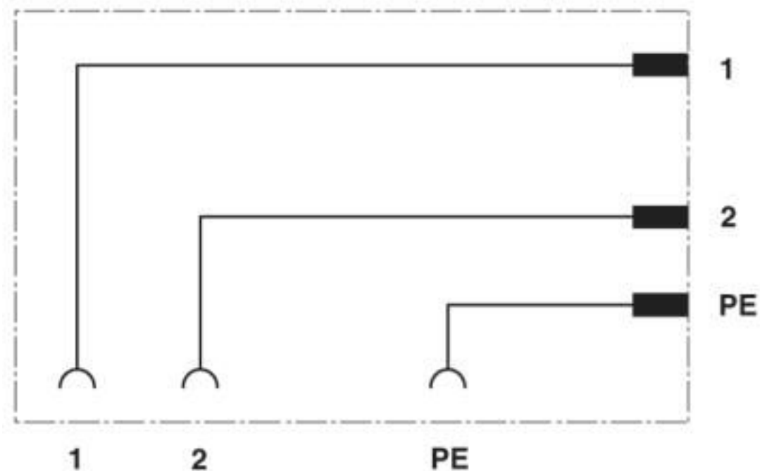
Circuit diagram
