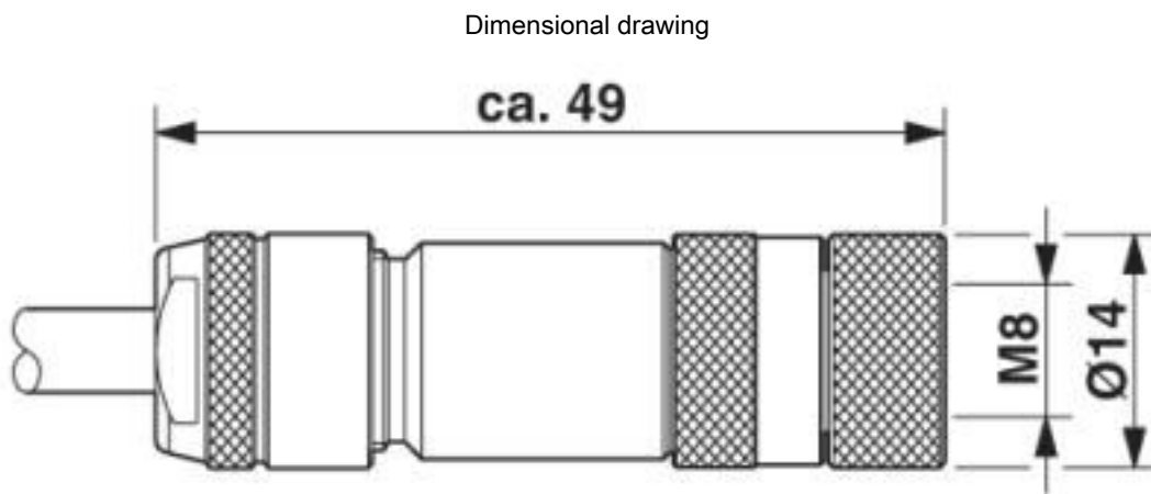
Socket M8 x 1, straight, shielded
