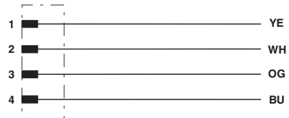
Circuit diagram
