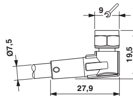
Dimensional drawing
