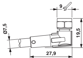
Dimensional drawing
