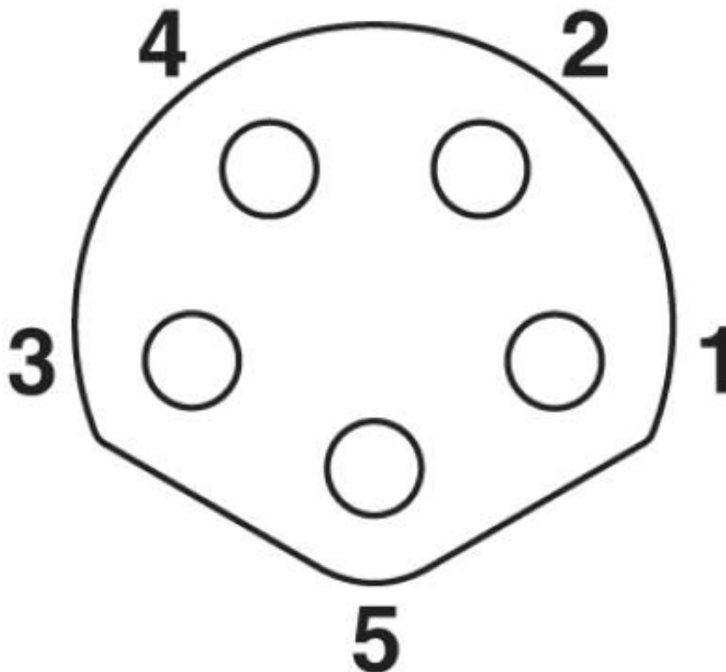
Pin assignment, socket side, M8, 5-pos., B-coded
