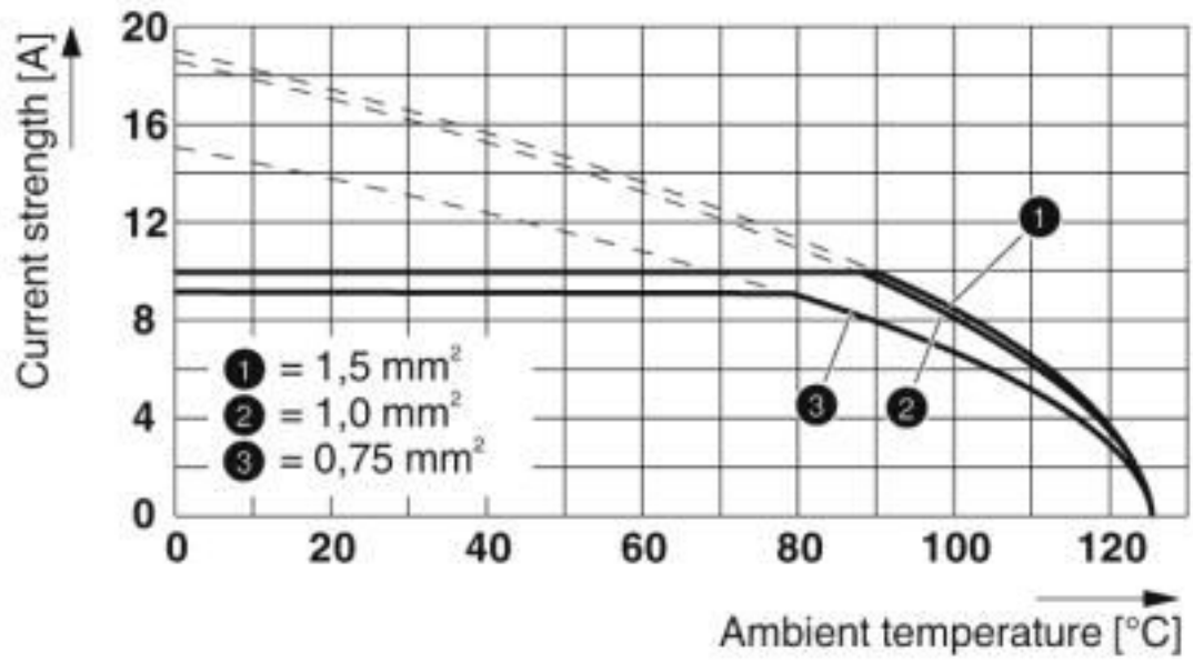
Derating diagram: Series HC-D 7-I-CT..
