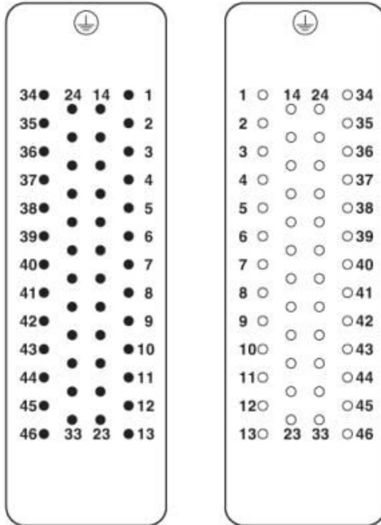
Schematic diagram
