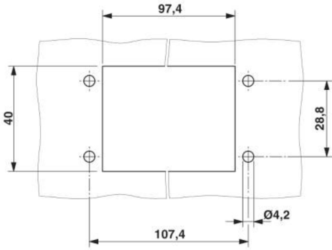
Mounting cutout for HC-B 24-ANDOCK-MOD...
