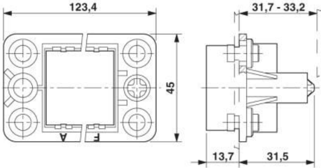
Dimensional drawing of HC-B 24-ANDOCK-MOD...
