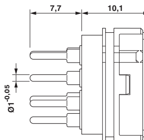
Dimensional drawing
