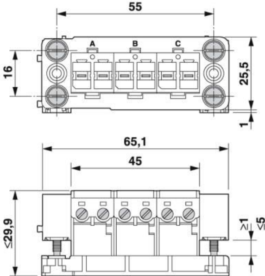
Dimensional drawing
