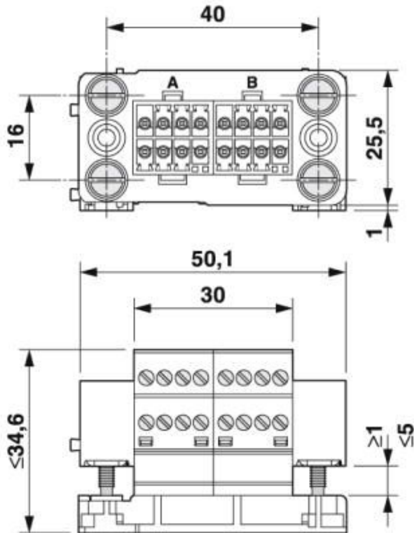
Dimensional drawing
