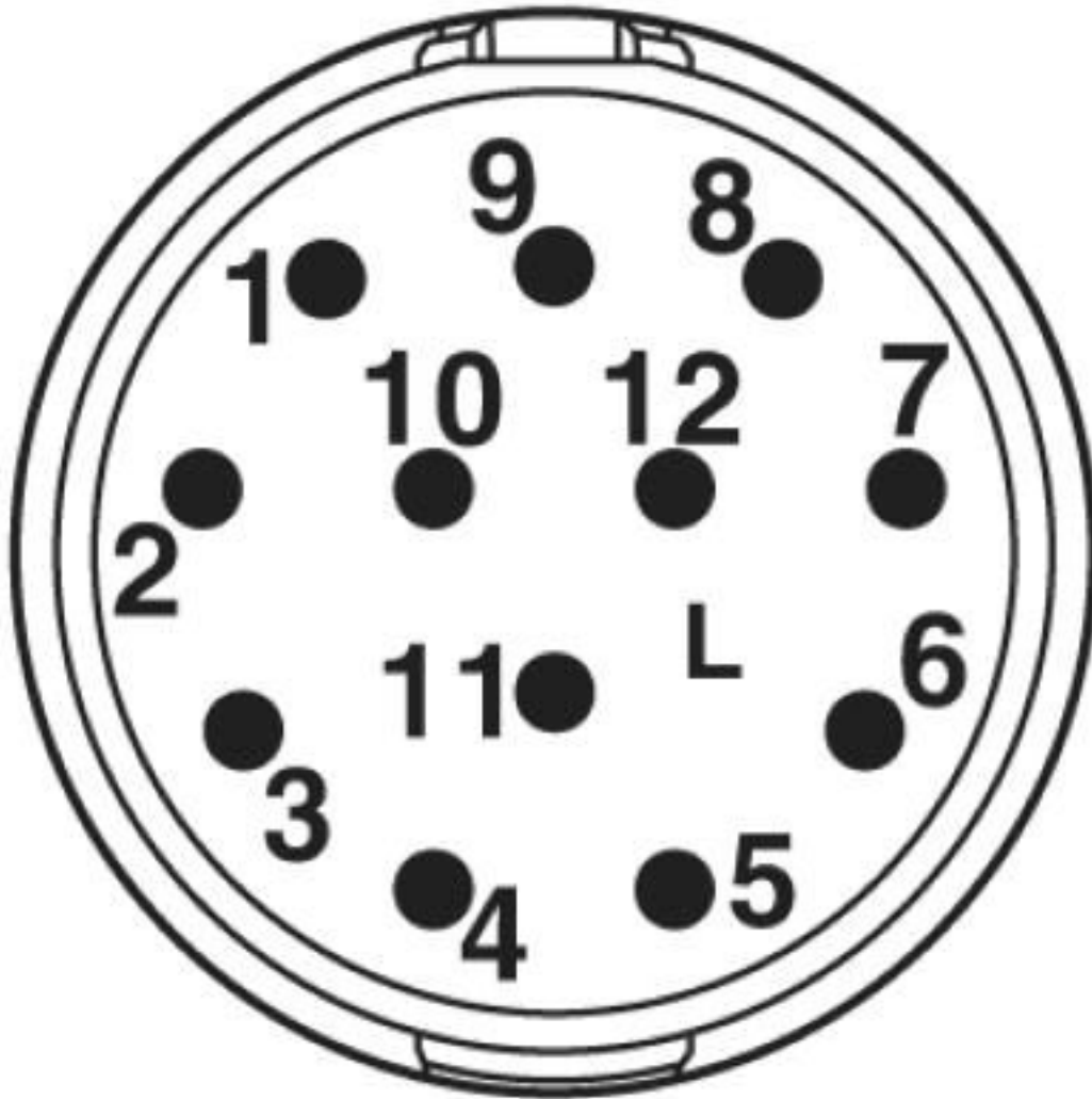
Contact chamber numbering (view of plug-in side), pin counter direction
