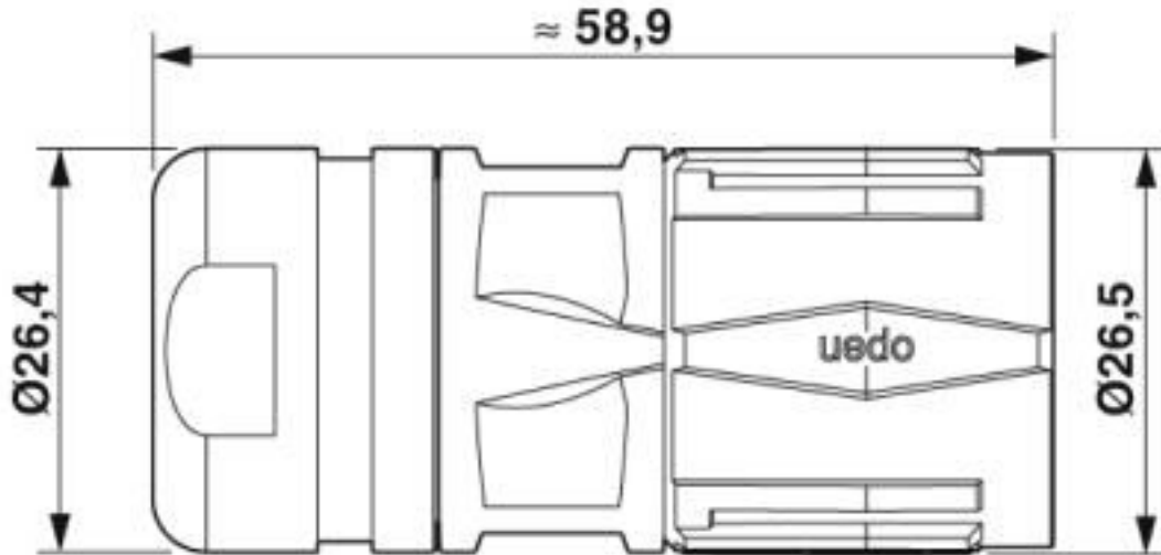
Schematic diagram
