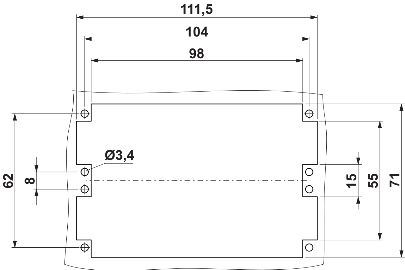
Dimensional drawing
