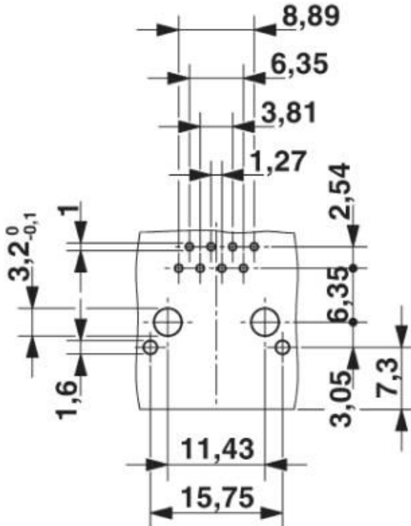
Drilling diagram
