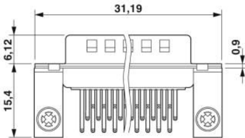
Dimensional drawing
