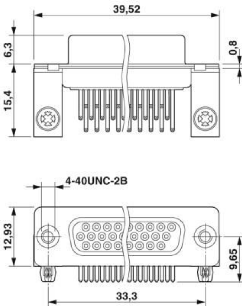
Dimensional drawing
