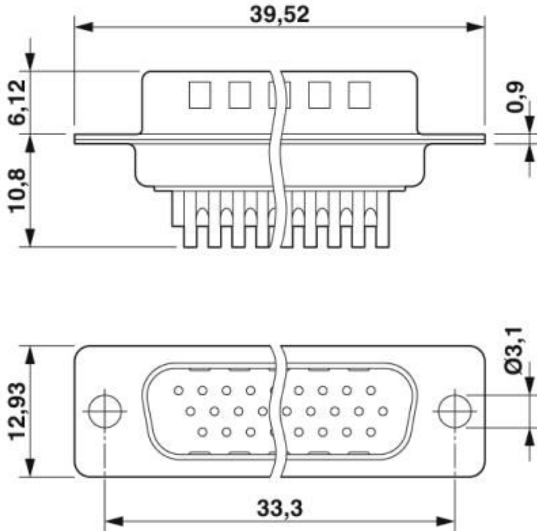
Dimensional drawing
