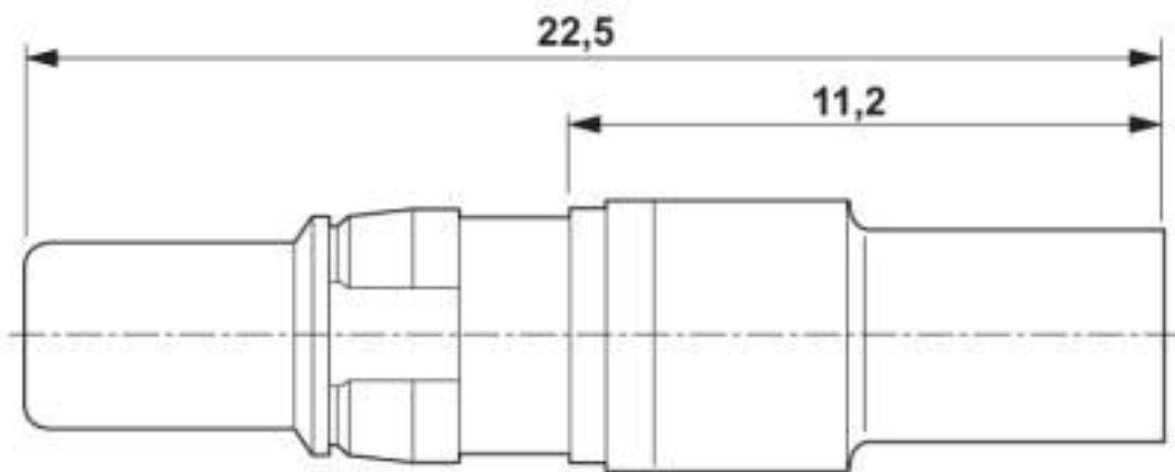
D-SUB coaxial contact pin
