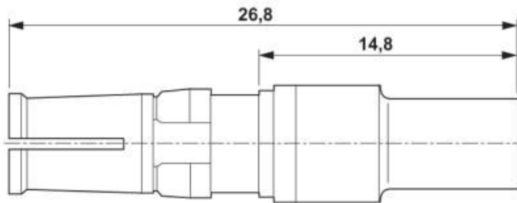
D-SUB coaxial contact socket
