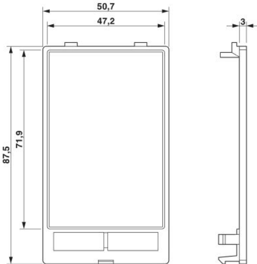
Dimensional drawing
