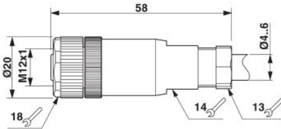
Dimensional drawing
