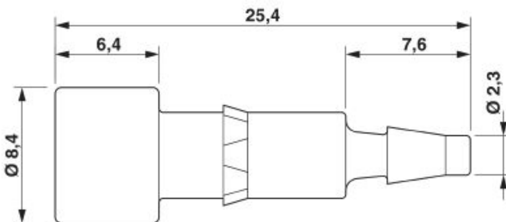
Dimensional drawing
