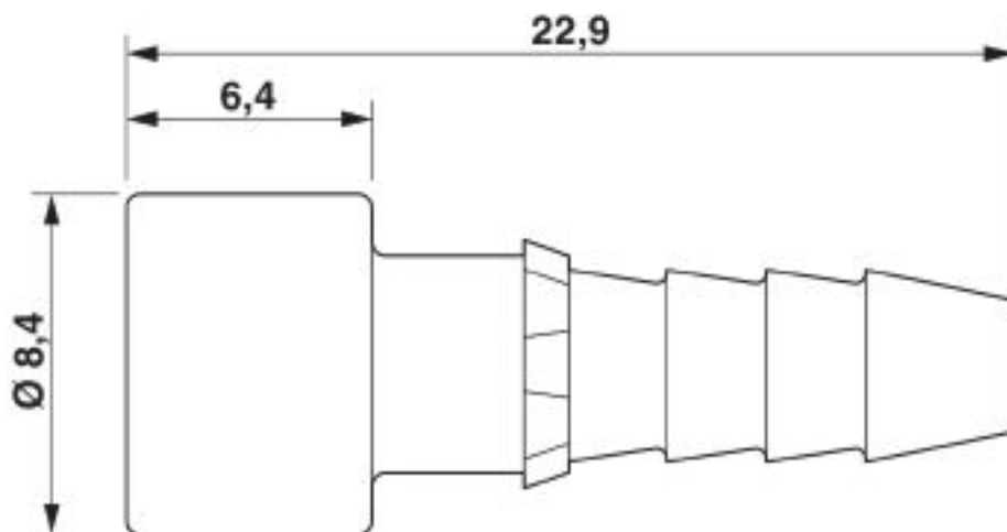
Dimensional drawing
