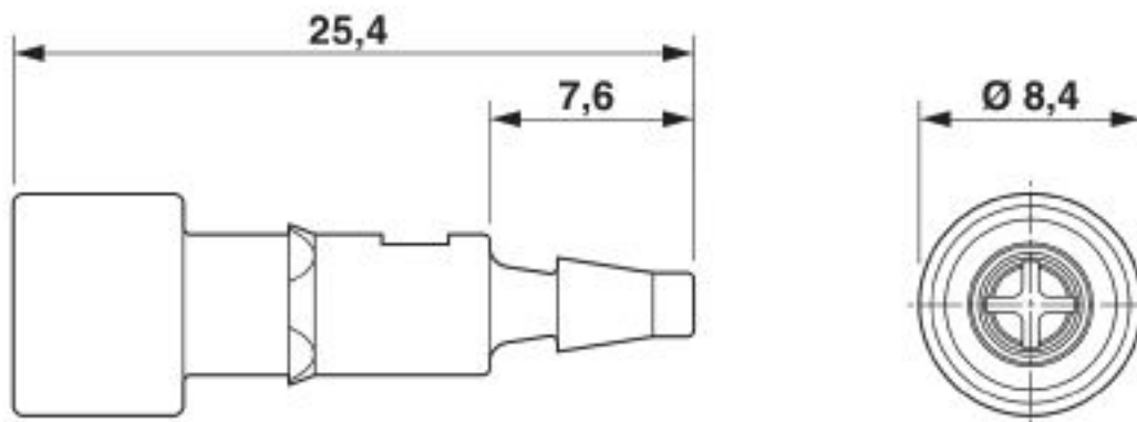
Dimensional drawing
