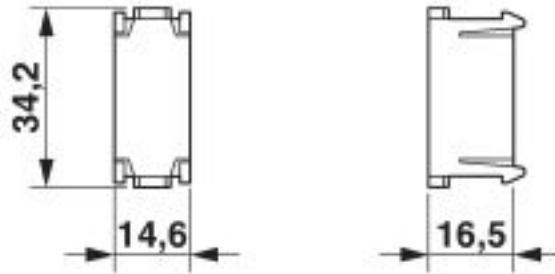
Dimensional drawing
