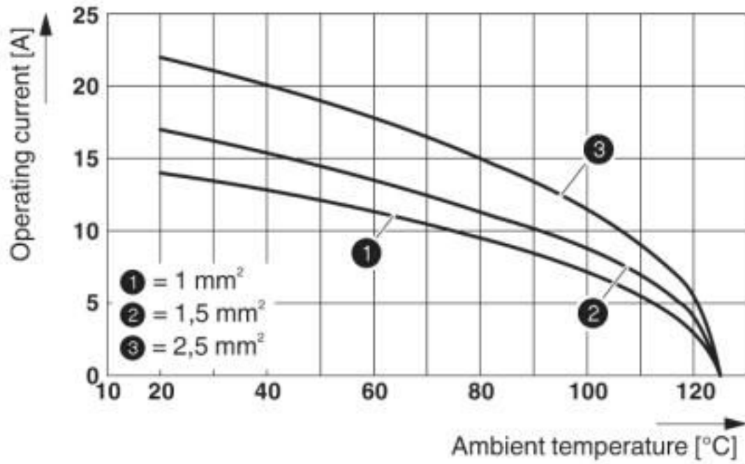
Derating diagram: Series A 16...S
