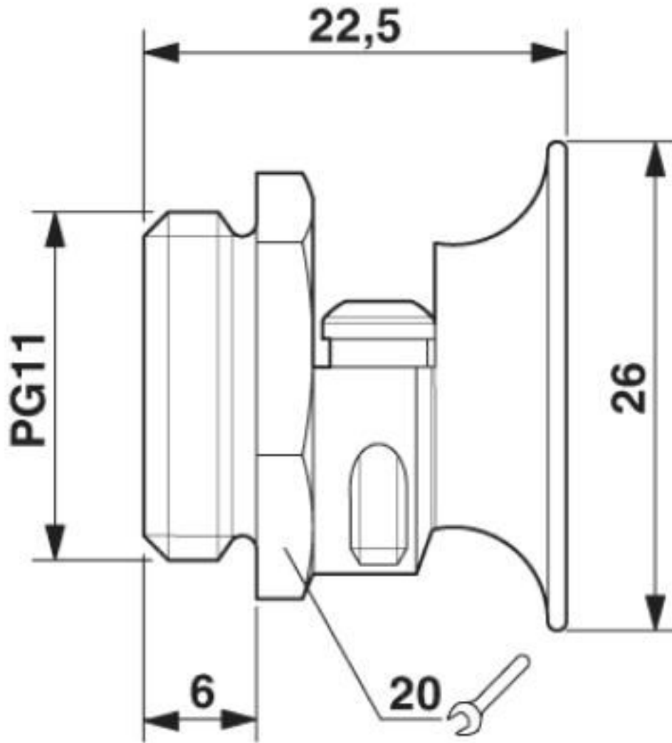
Dimensional drawing
