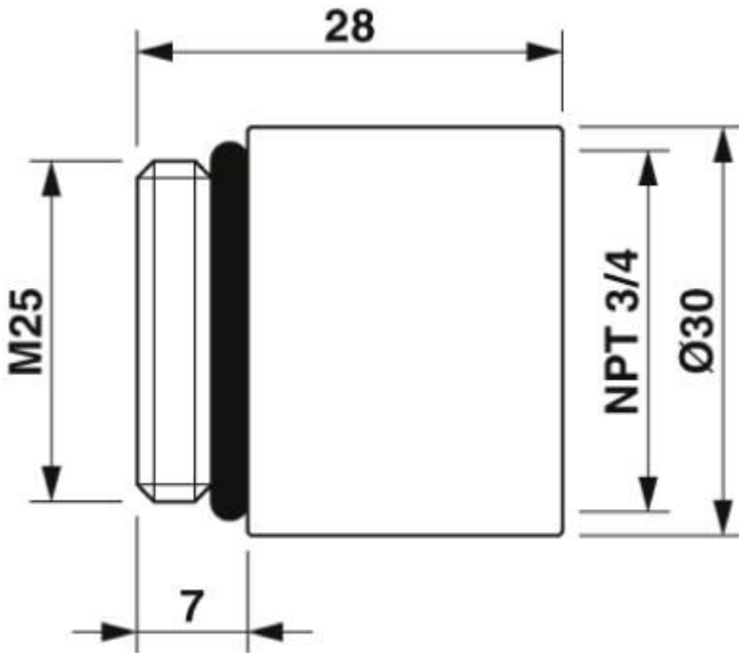
Dimensional drawing
