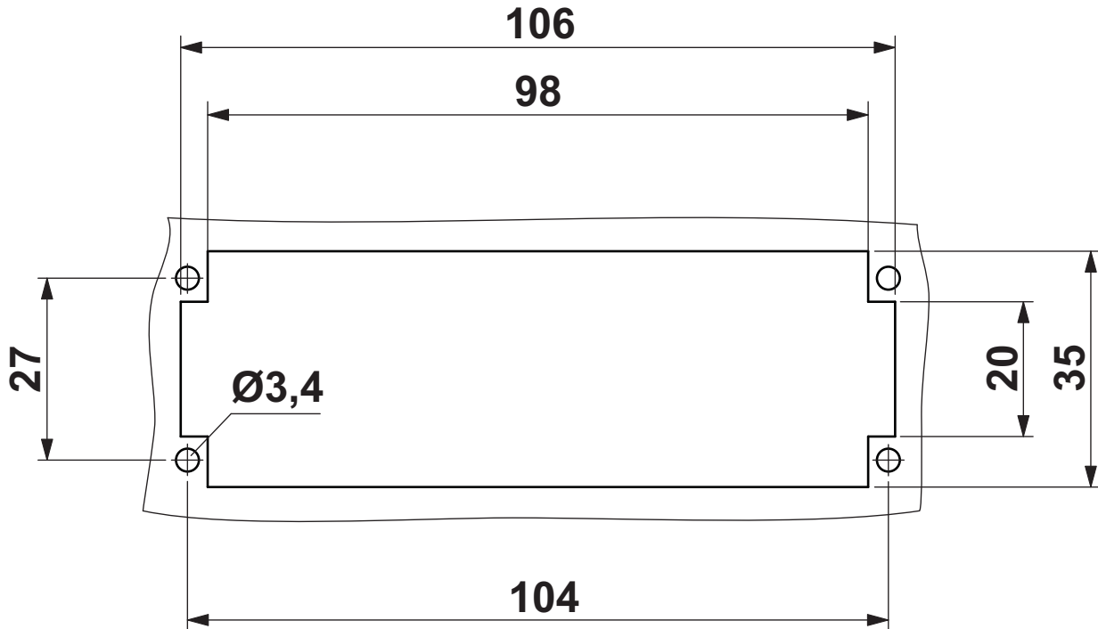
Mounting cutout
