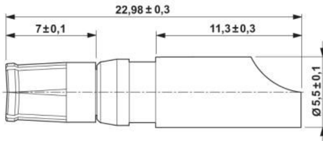
Dimensional drawing
