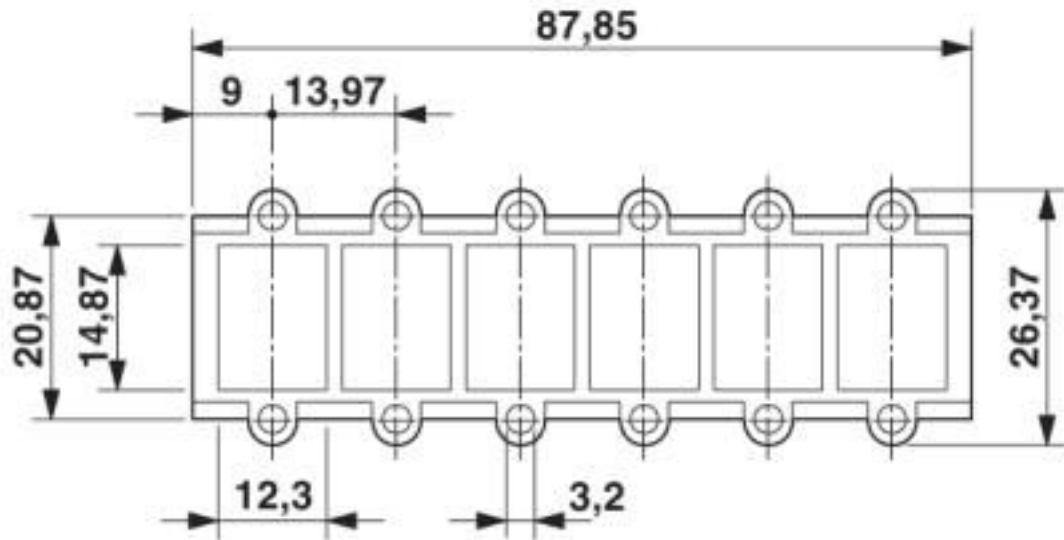
RJ45 panel mounting frame, IP20
