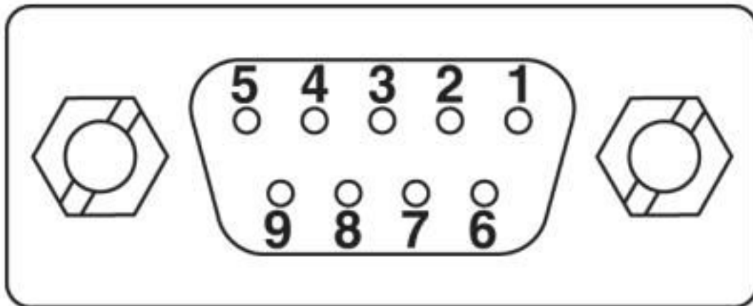
Schematic diagram
