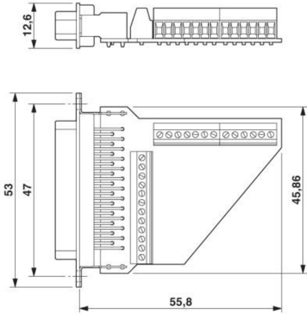
Dimensional drawing
