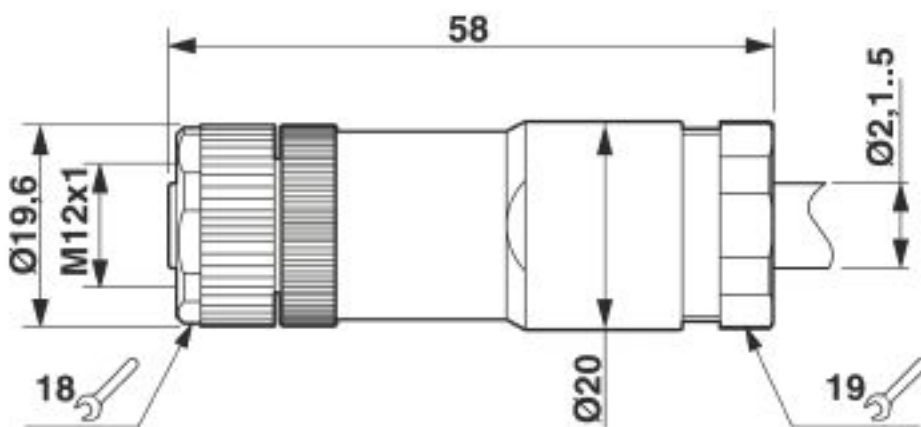
Dimensional drawing
