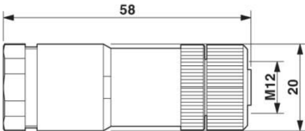
Dimensional drawing
