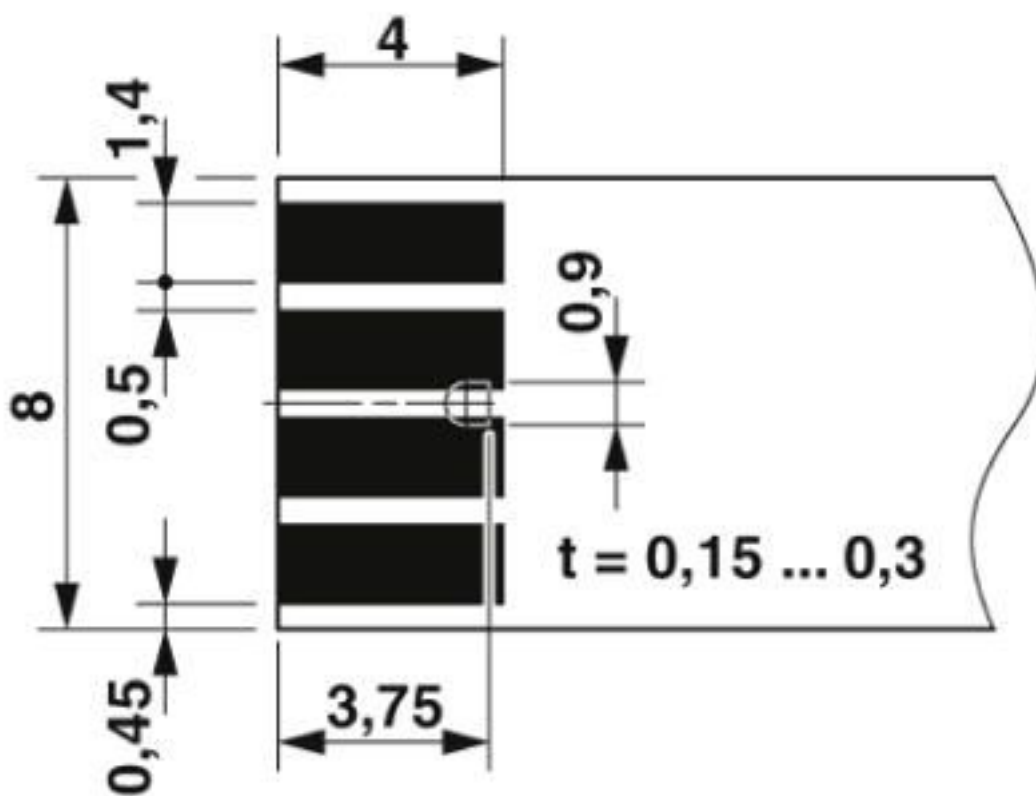
Drilling diagram
