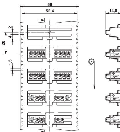
Dimensional drawing
