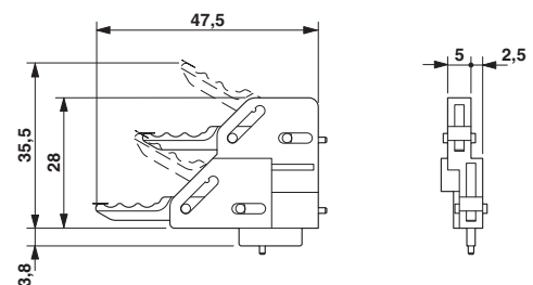
Dimensional drawing
