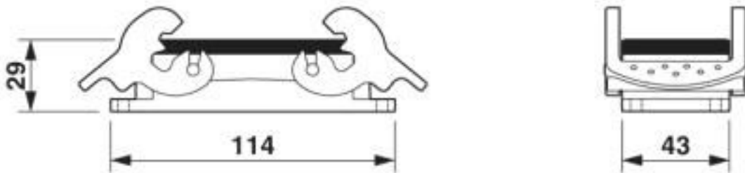
Dimensional drawing
