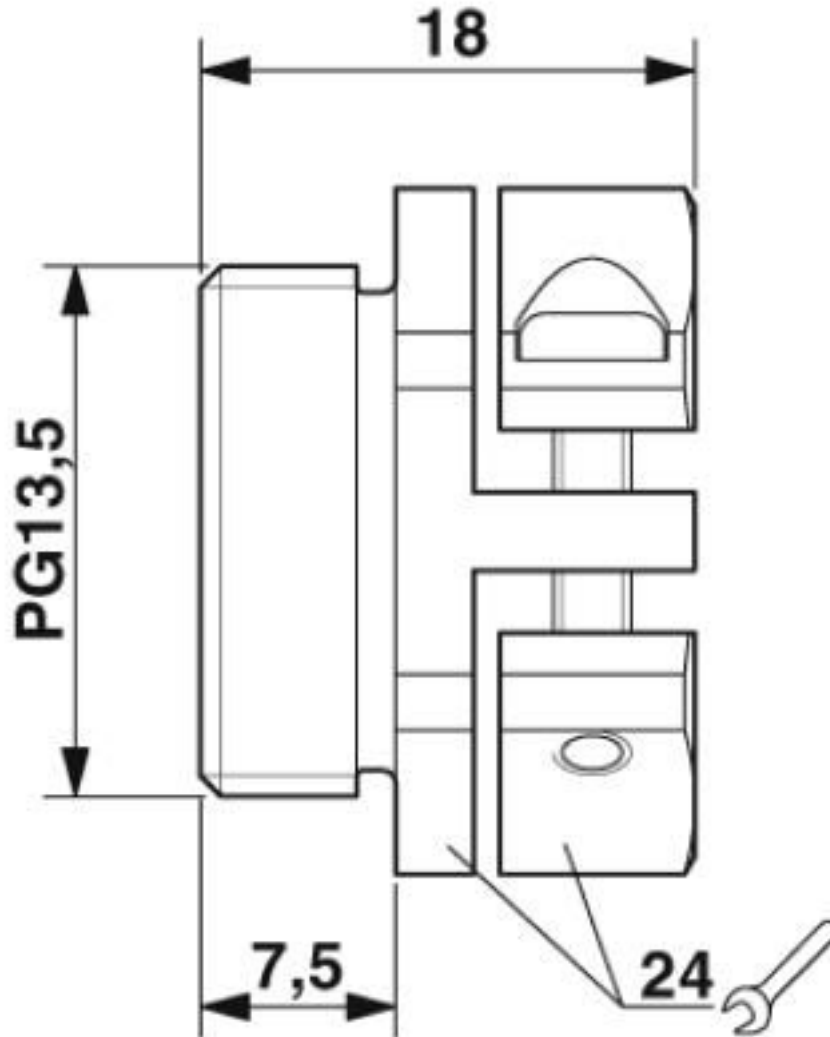
Dimensional drawing
