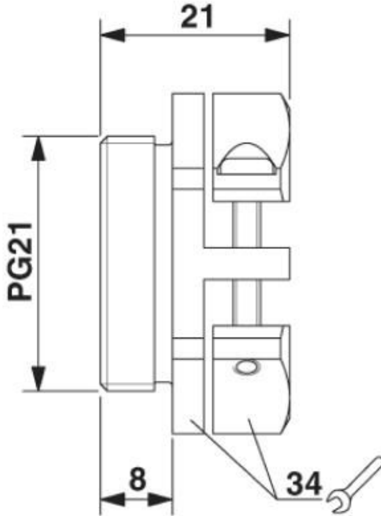
Dimensional drawing
