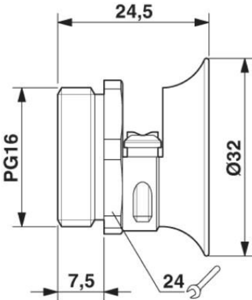
Dimensional drawing
