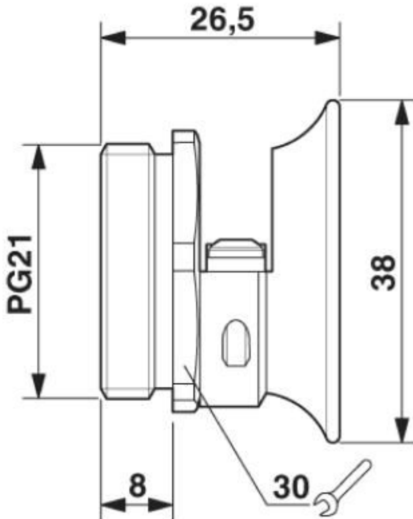
Dimensional drawing
