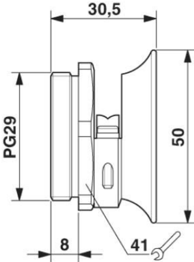
Dimensional drawing
