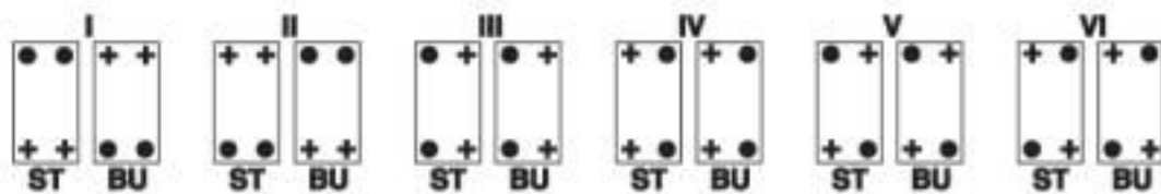
Coding for housings with one contact insert
