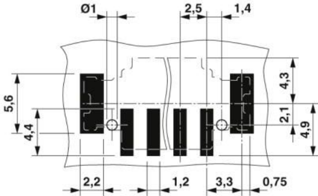
Drilling diagram
