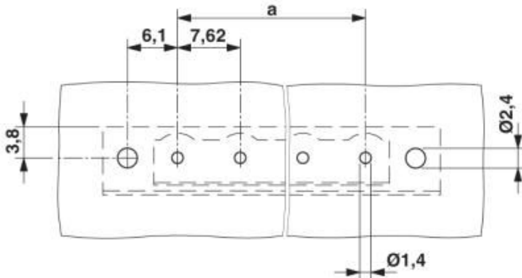
Drilling diagram
